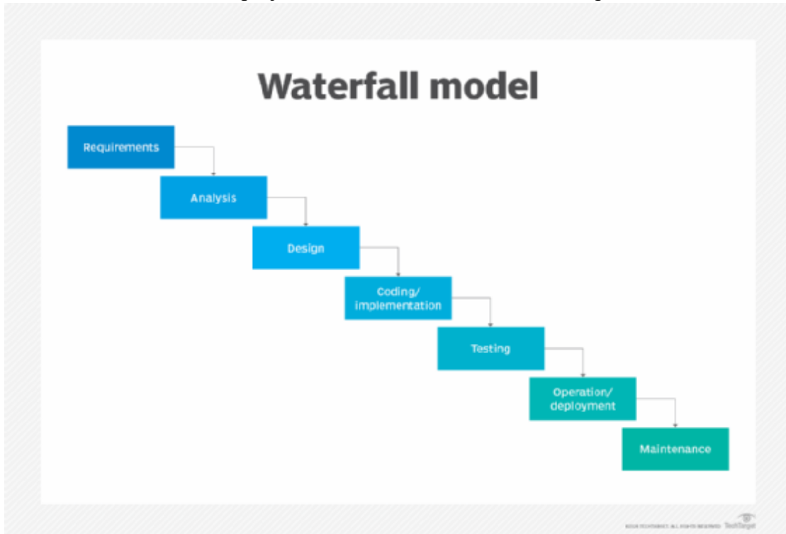
Figure 2 Waterfall model
